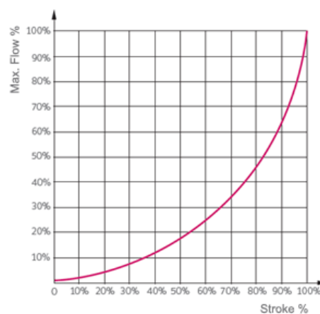
Opening Flow Characteristic Equal-percentage
